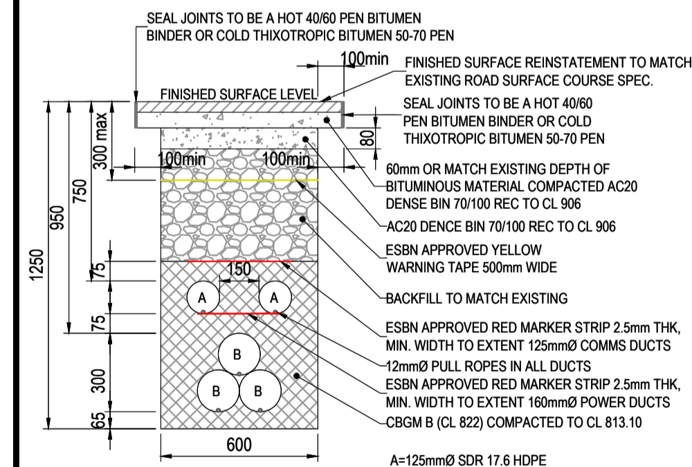
DETAIL 02 TRENCH FOR 160mm DUCTS IN TREFOIL FORMATION IN ROADWAYS SCALE 1:20
