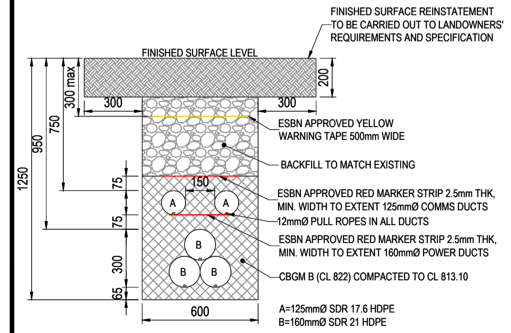
DETAIL 01 TRENCH FOR 160mm DUCTS IN TREFOIL FORMATION IN RESERVATION SCALE 1:20
